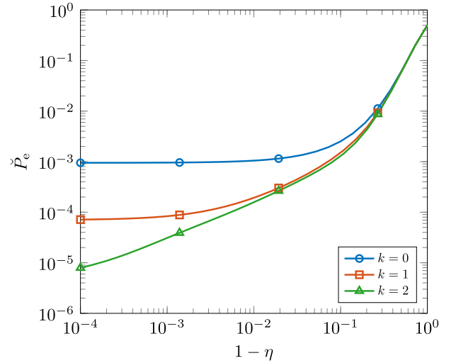
Fig. 8. MDEP for the discrimination between a noisy PACS and the thermal state affected by photon loss as a function of \eta , with n_p = 6 , \bar{n} = 10^{-2} , and p_0 = p_1 = 1/2 .
